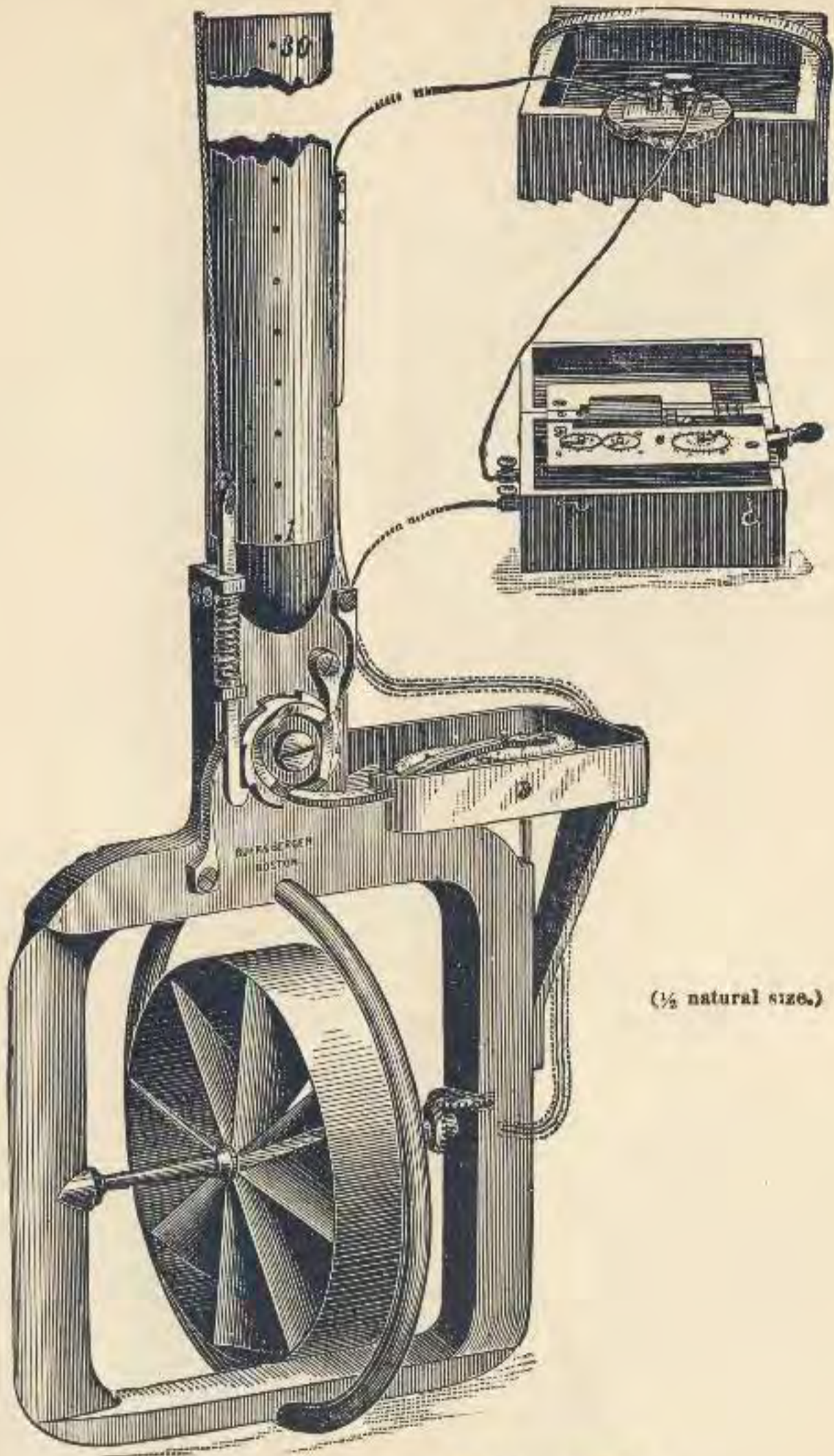
Current Meters No. V and VI. As made by Buff & Berger.
