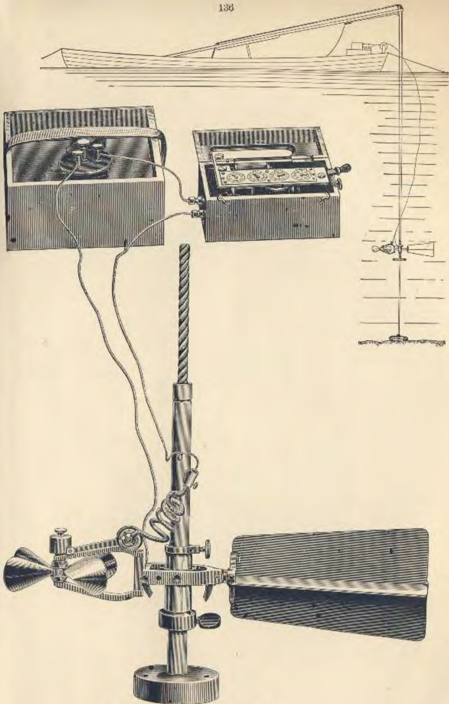
Current Meter No. IV.
