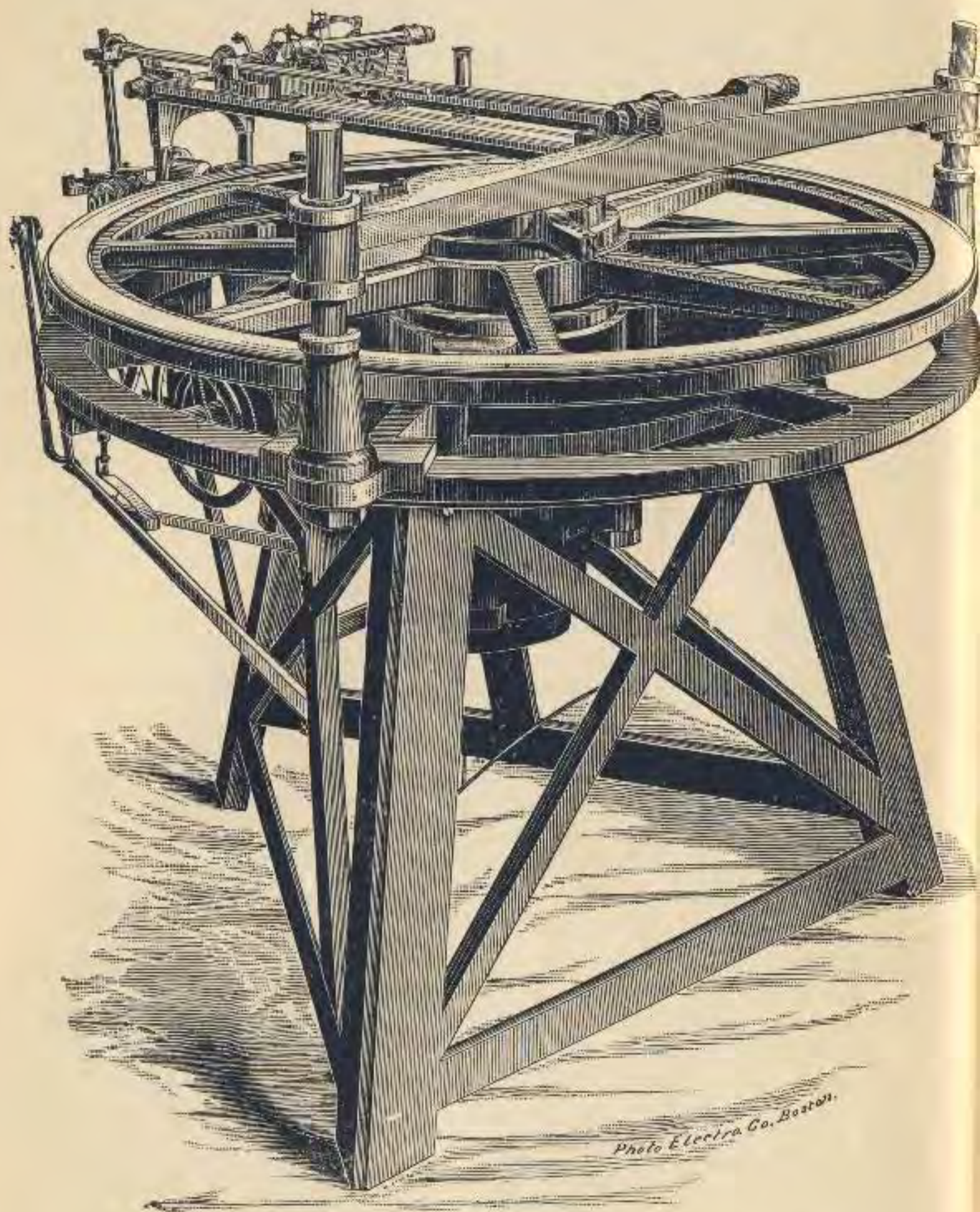
Buff & Berger's Large Automatic Dividing Engine.
