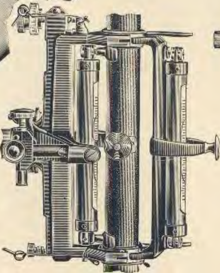
Auxiliary Striding Level.
