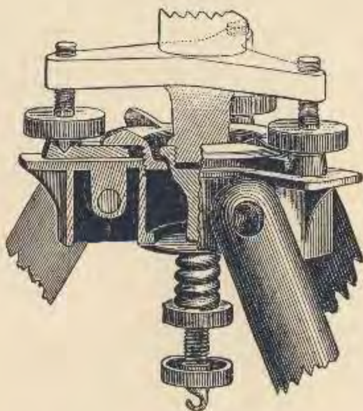
Shifting Center for a Transit with Three Leveling Screws.
