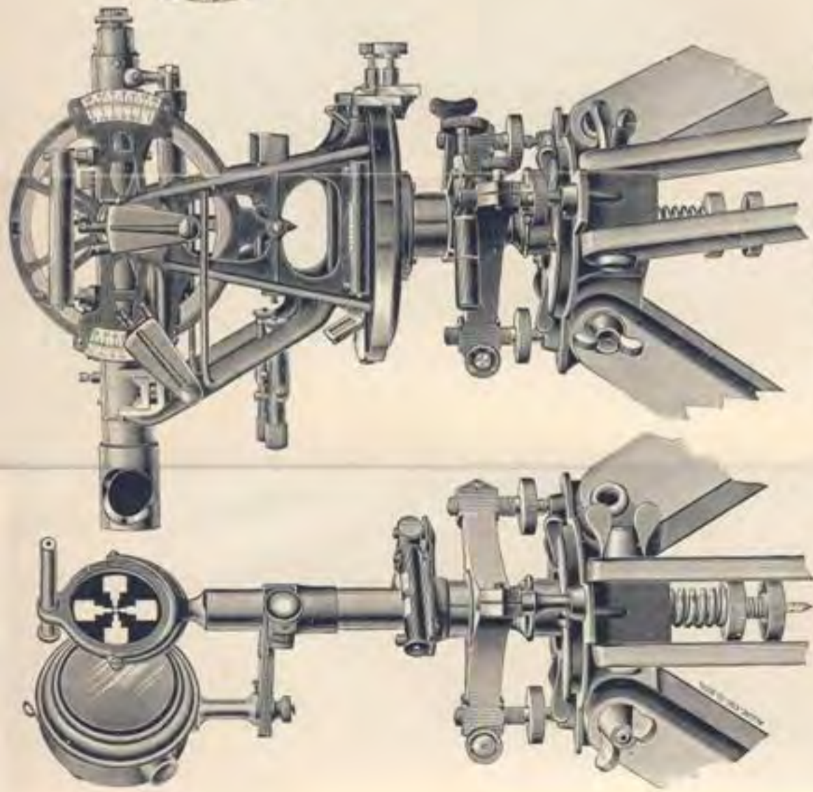
Instrument with Telescope in Normal Bearings.
