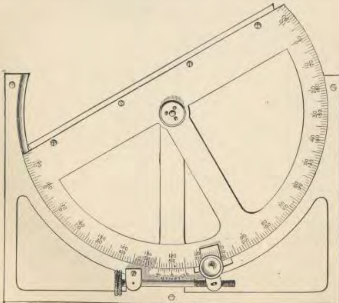
CROZET'S PROTRACTOR. 1488.
