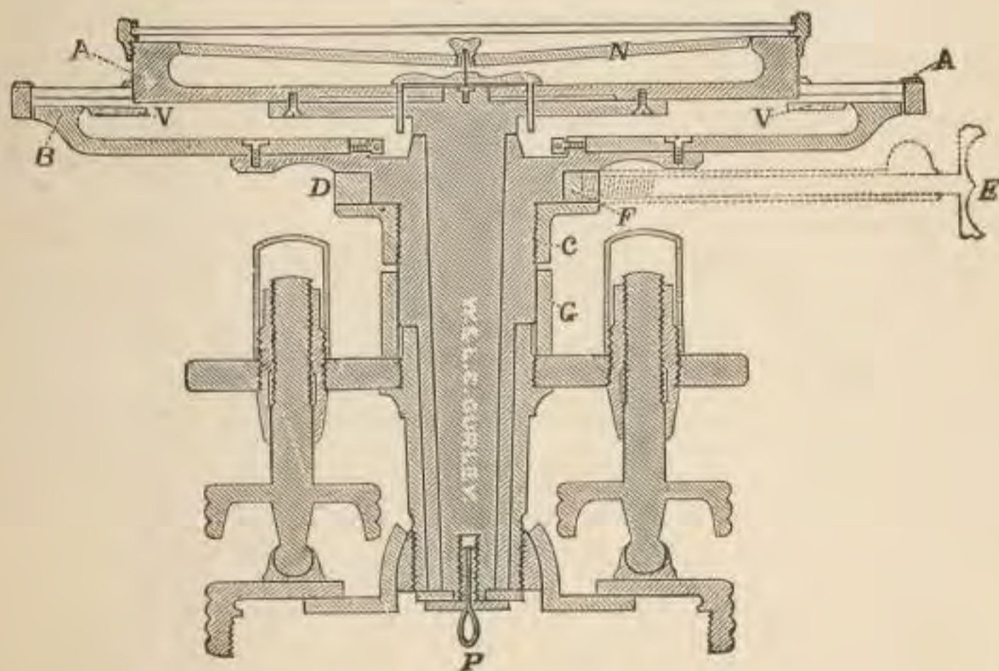
THE SOCKETS AND CIRCULAR PLATES.
