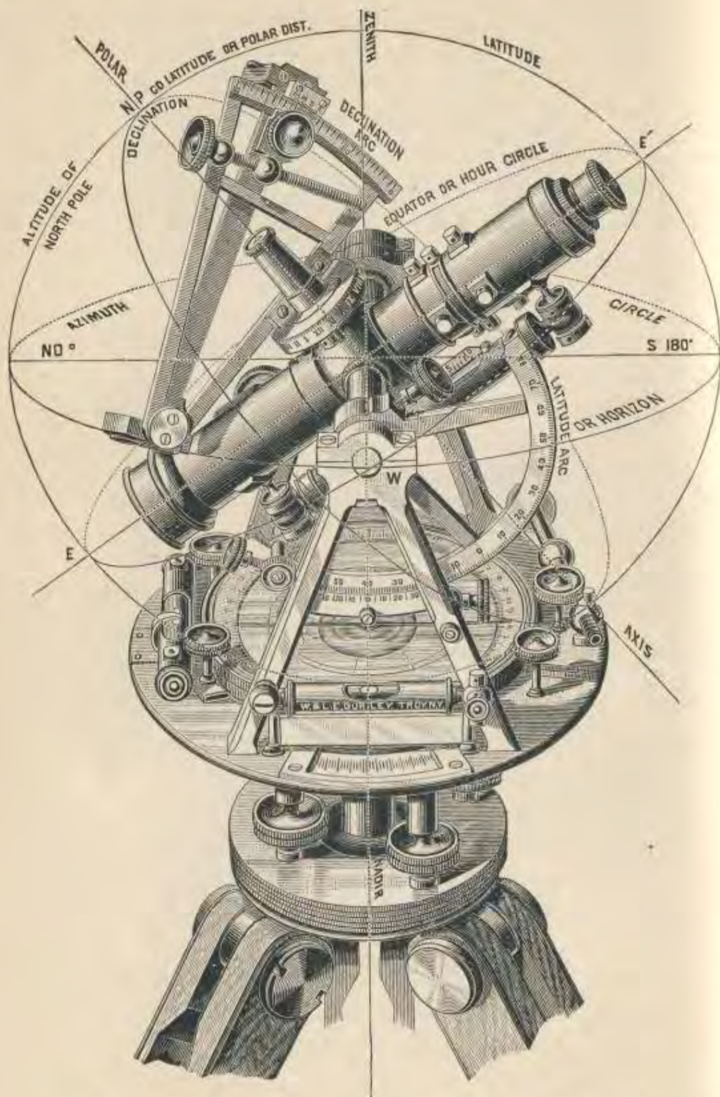
GRAPHIC ILLUSTRATION OF THE SOLAR APPARATUS.
