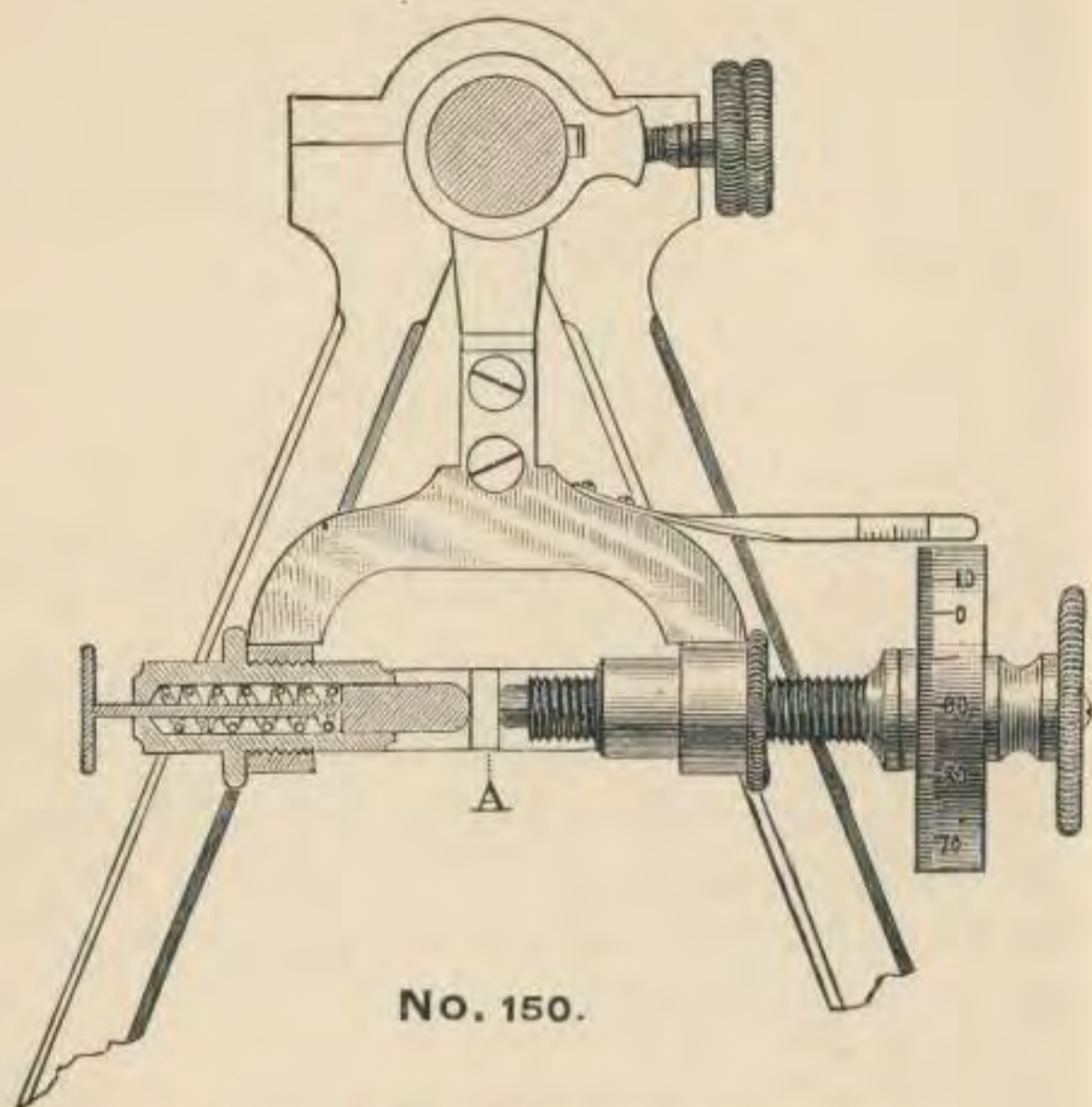
GRADIENTER ATTACHMENT. Price, $18.00.
