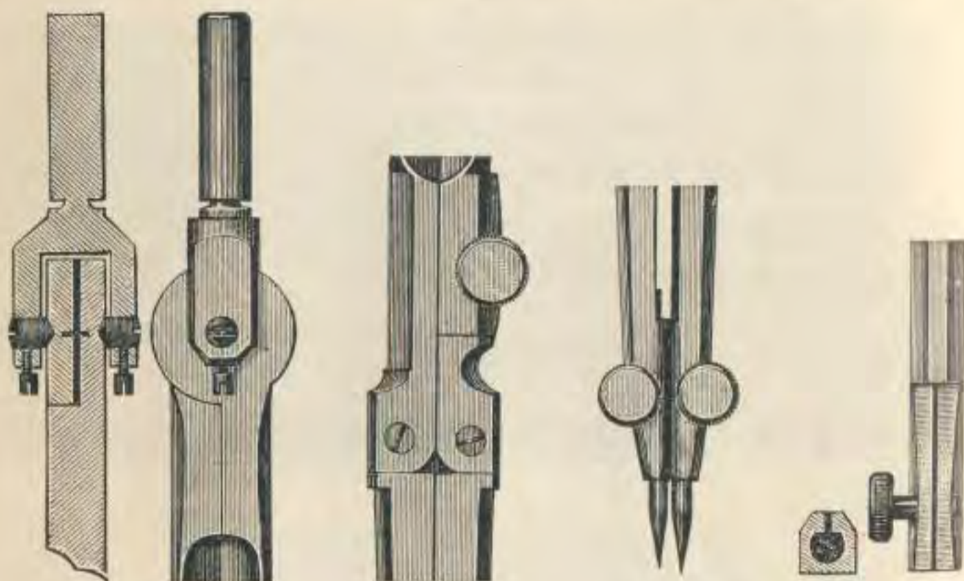
Alteneder's Patent Joint.
