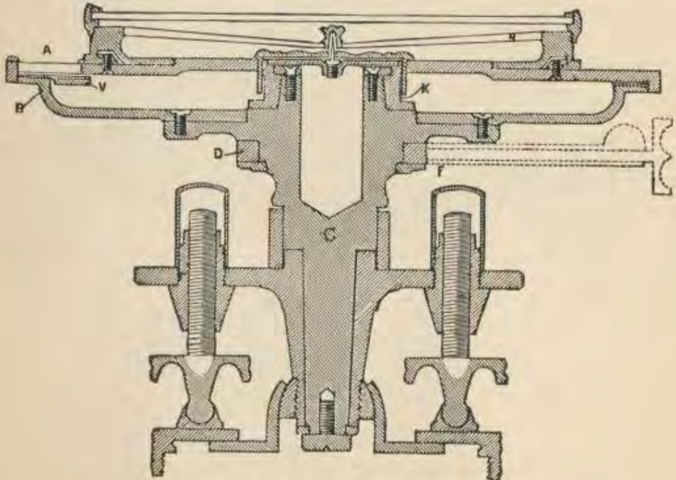
THE SOCKETS AND CIRCULAR PLATES.
