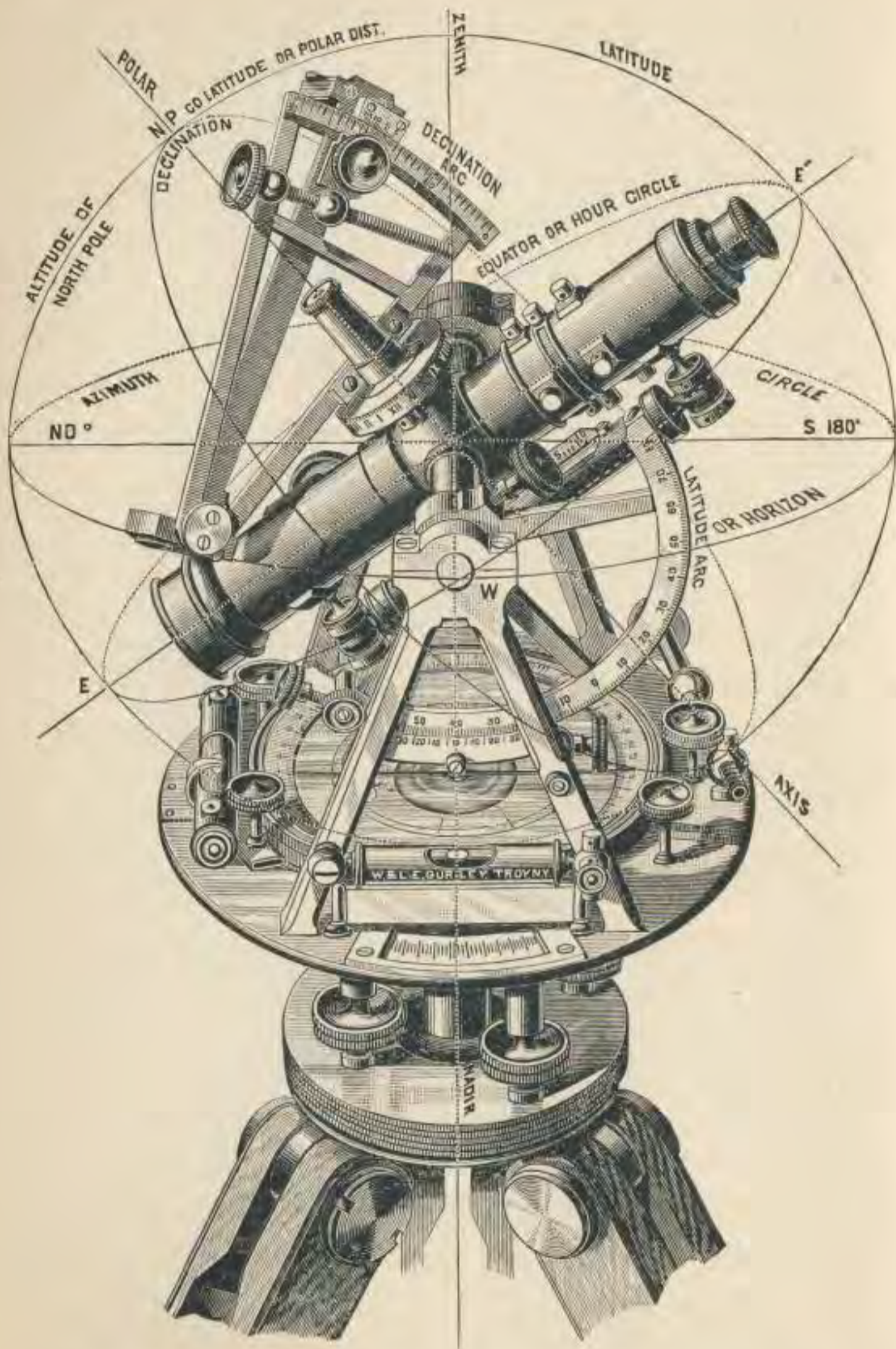
GRAPHIC ILLUSTRATION OF THE SOLAR APPARATUS
