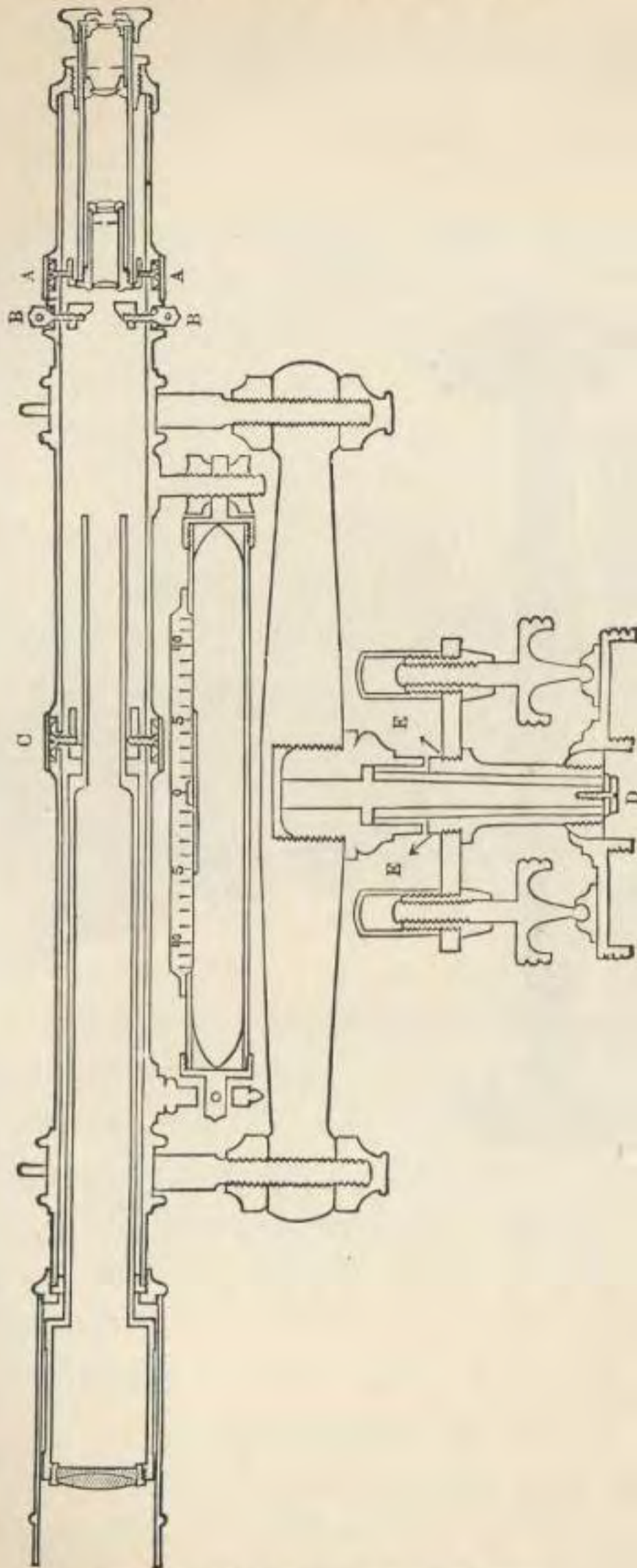
SECTIONAL VIEW OF Y LEVEL
