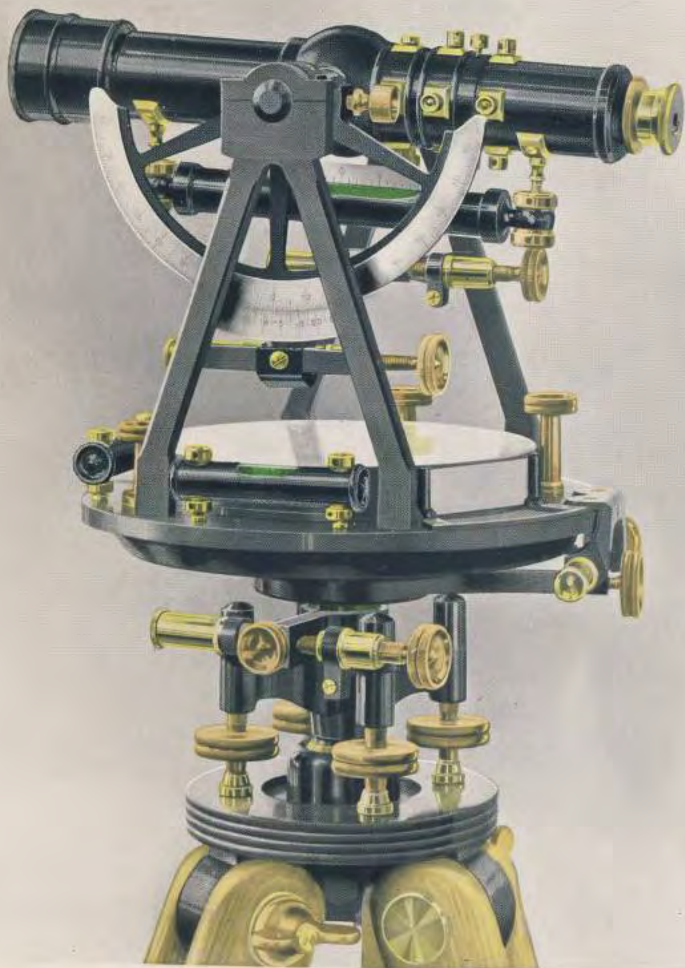
LIGHT MOUNTAIN TRANSIT No. 28
