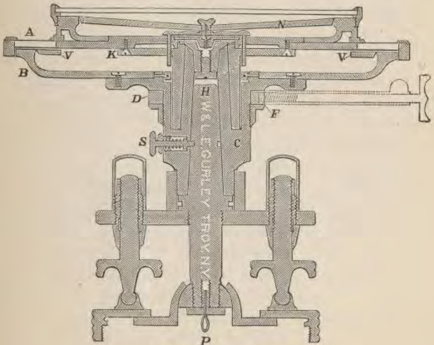
SOCKETS AND CIRCULAR PLATES
