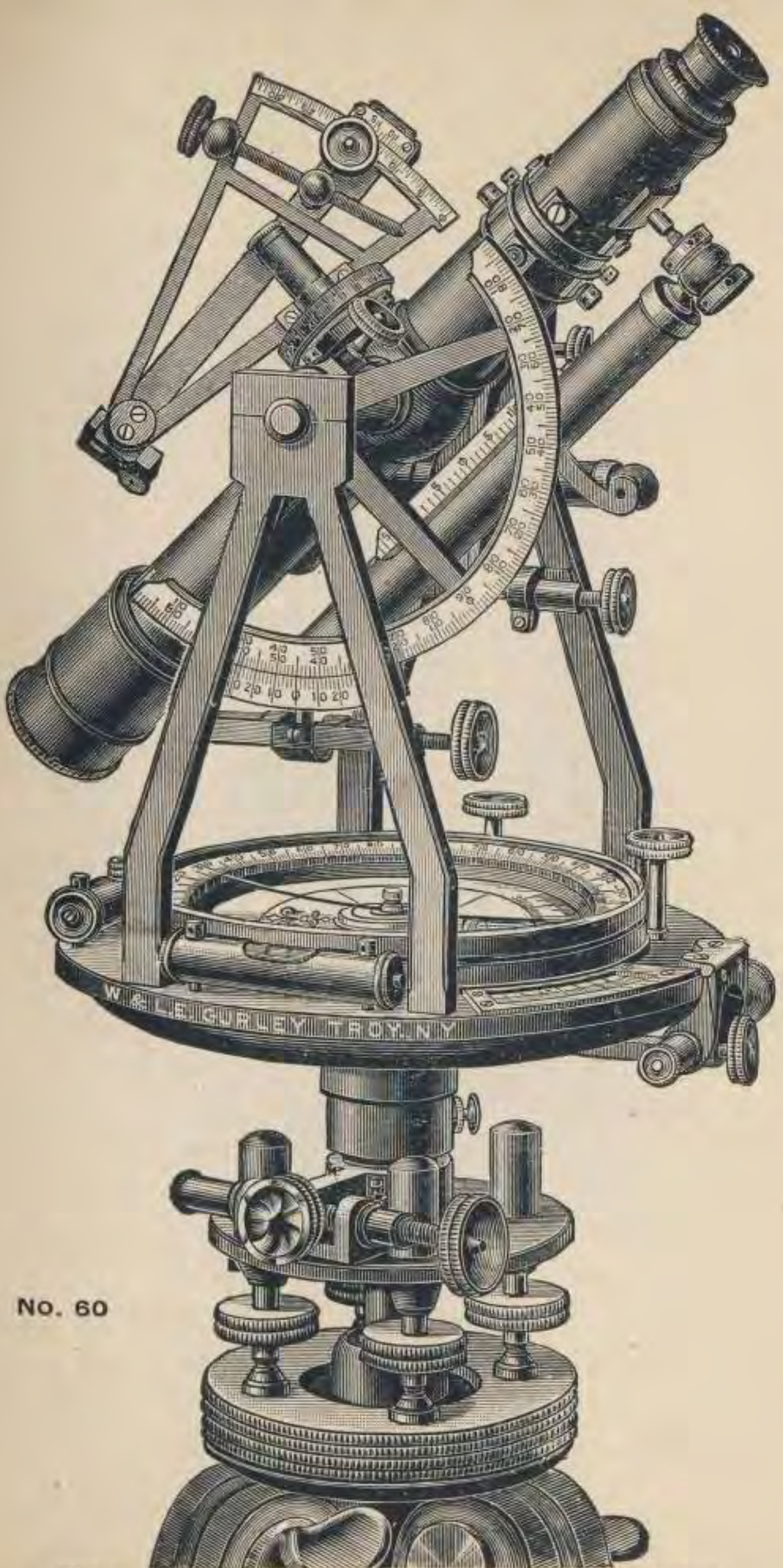
SURVEYORS' TRANSIT WITH SOLAR ATTACHMENT
