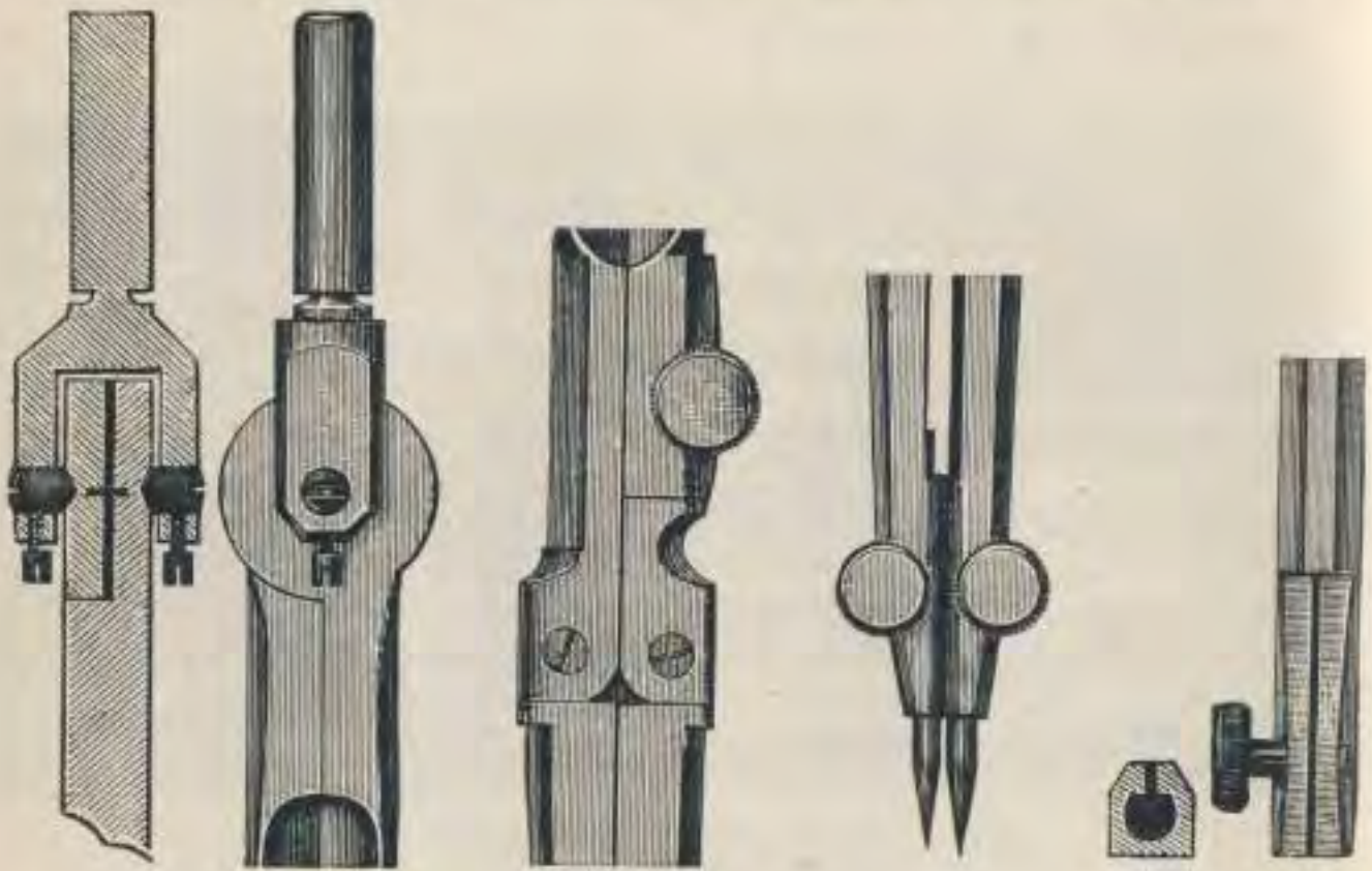
Alteneder's Patent Joint
