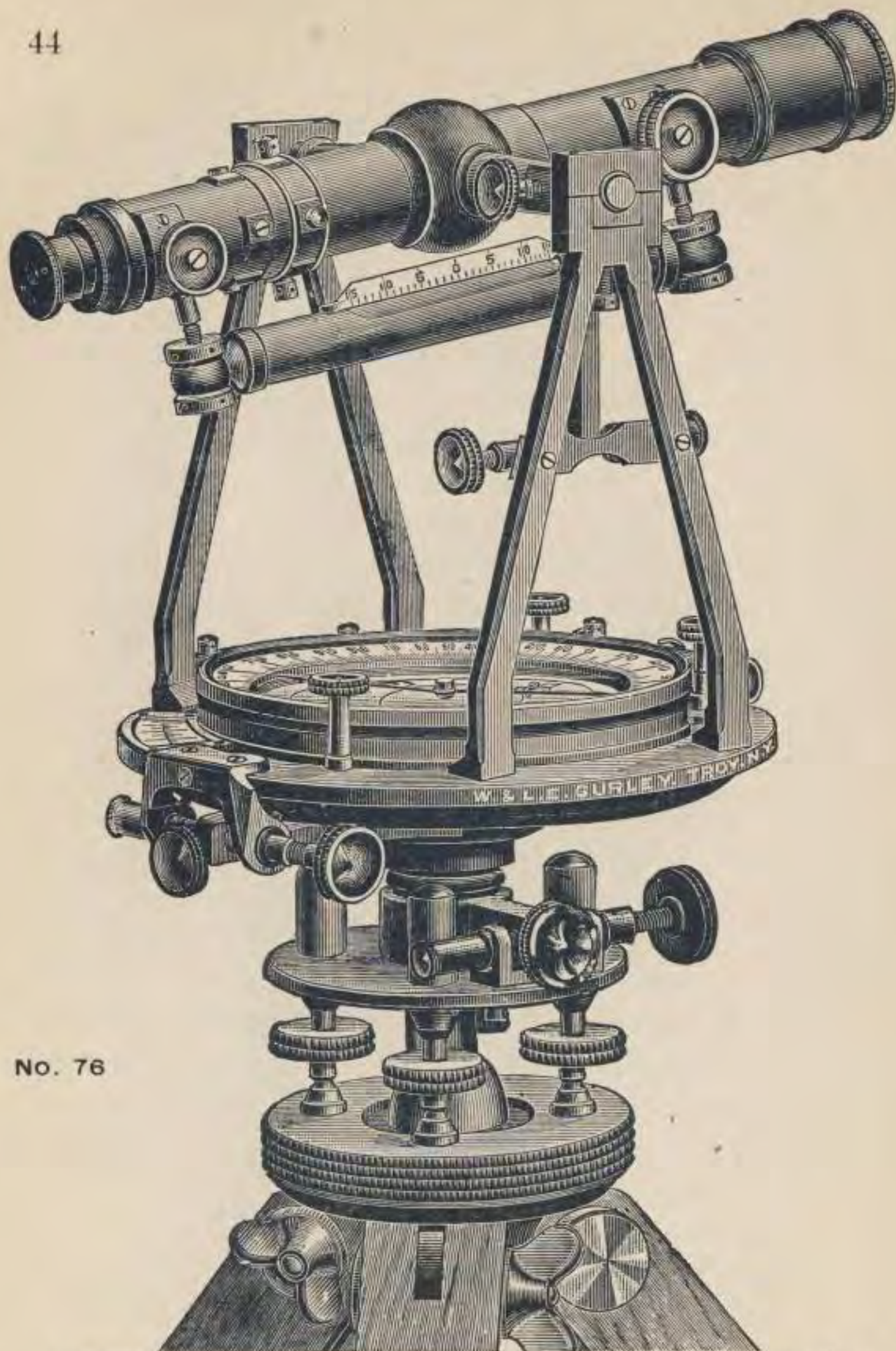
Surveyors' Transit, one vernier to limb, 5-inch needle, with level on telescope, clamp and tangent to telescope axis, and tripod. Price, $133.00.
