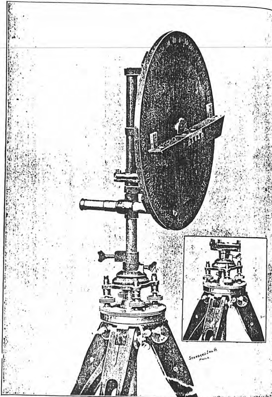
Made by Heller & Brightly, Philadelphia, Pa. The small figure shows the Removable Leveling Arrangement
