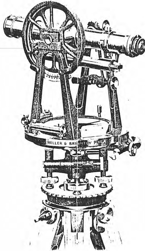
MODEL NO. 4C 6¼ in. at Reading Edge
