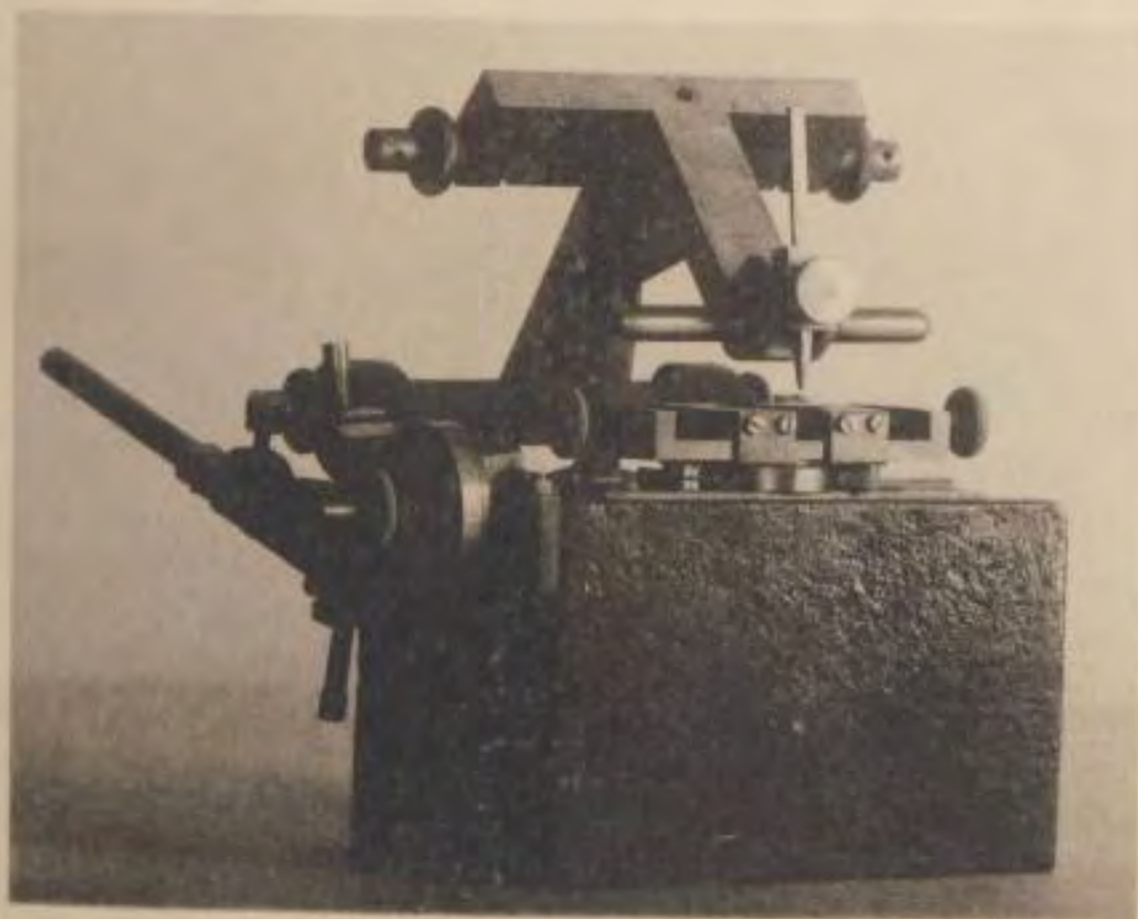
LINEAR DIVIDING ENGINE, IN GRADUATING DEPARTMENT.
