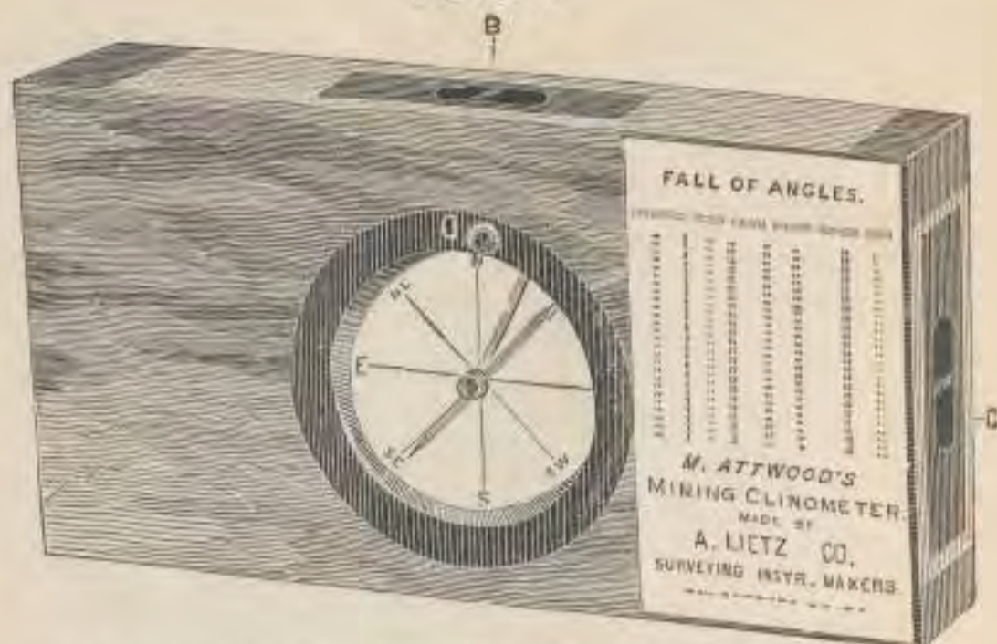
Attwood's Clinometer, showing Compass.
