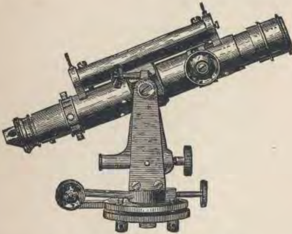
SAEGMÜLLER SOLAR ATTACHMENT.
