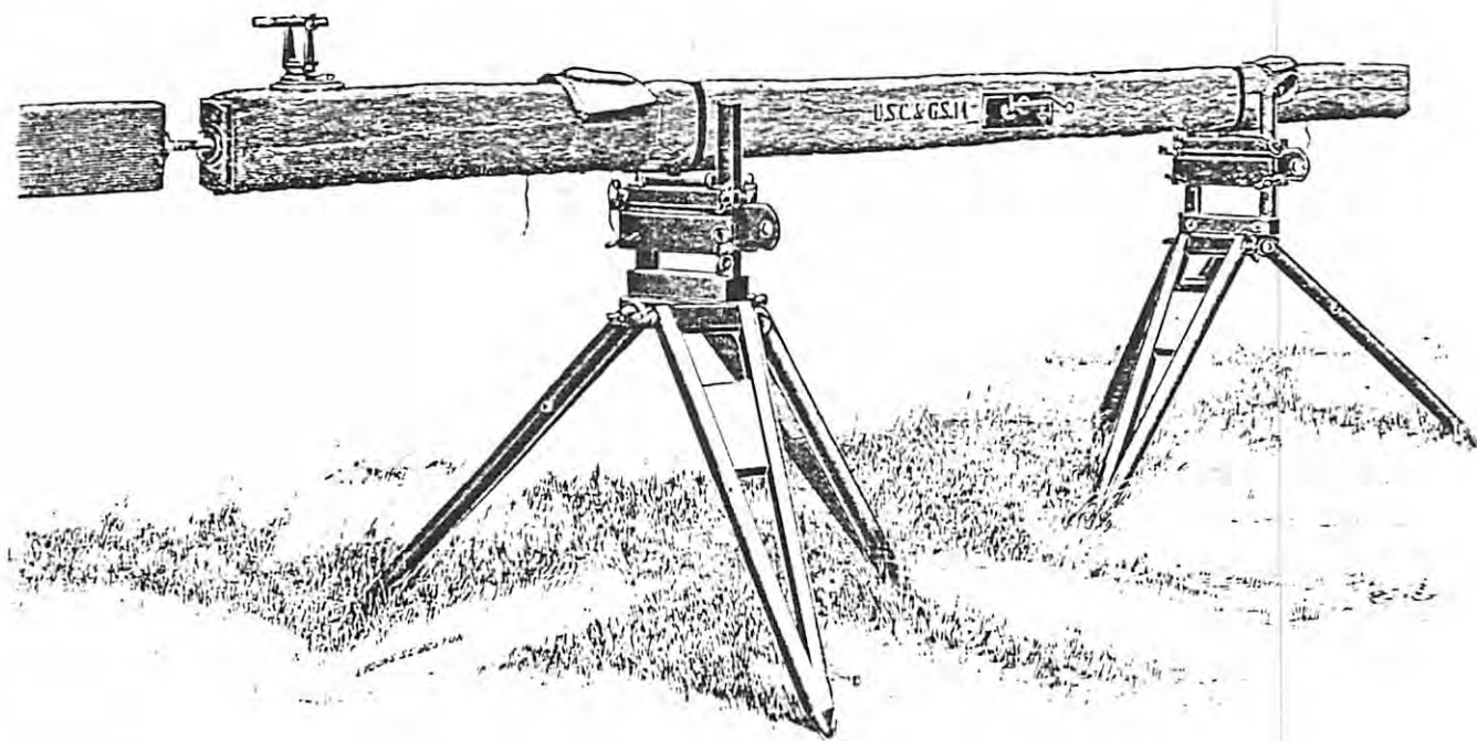
Improved Coast Survey Base Apparatus.
