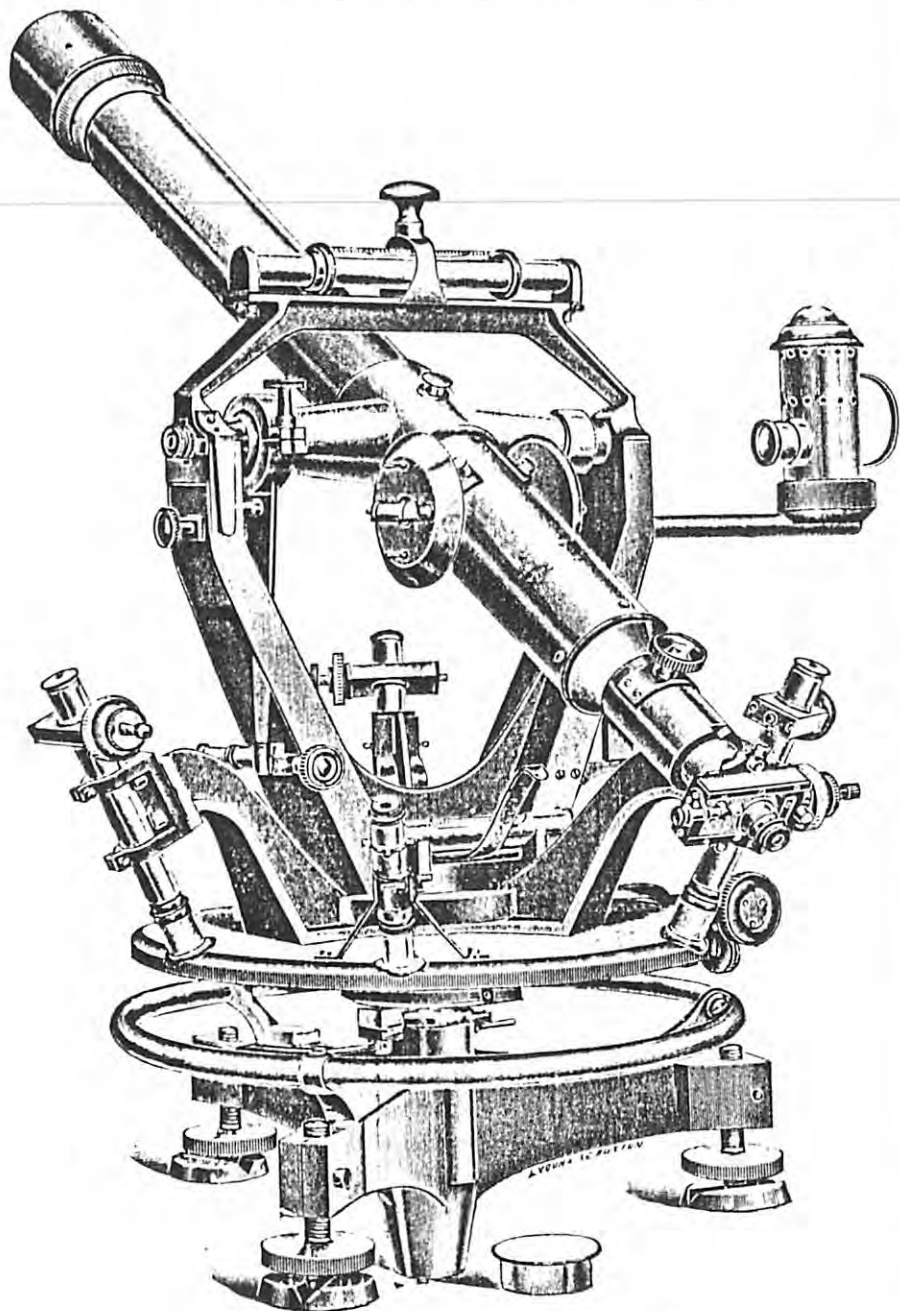
12-inch Coast Survey Theodolite.
