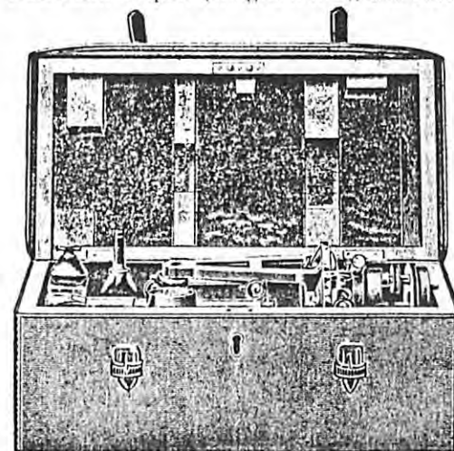
Mode of Packing 4-inch Mining Transit.
