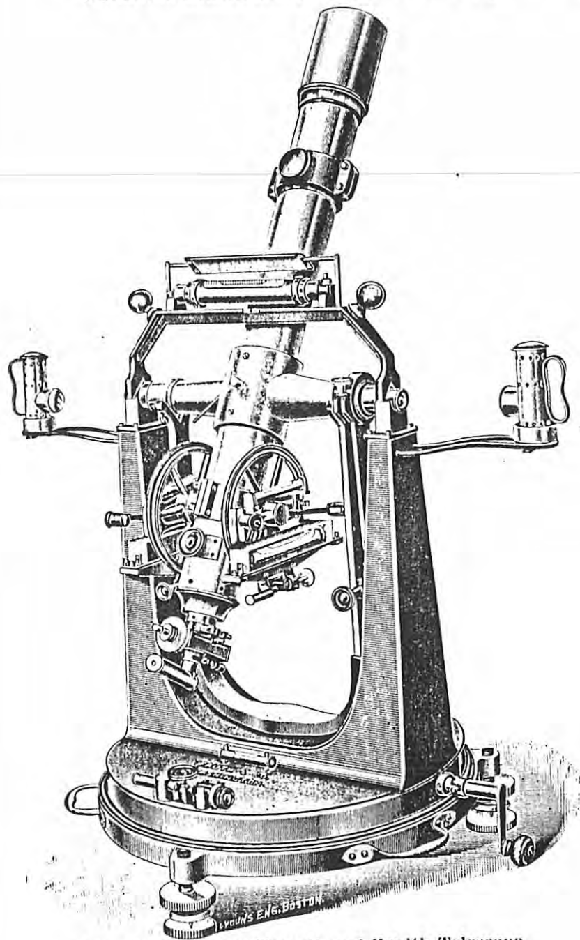
New Combination Transit and Zenith Telescope.
