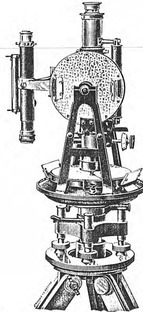
5-inch and 6-inch Mining Transit, No. 3, with full vertical circle and double opposite verniers, level, clamp, and tangent to telescope.
