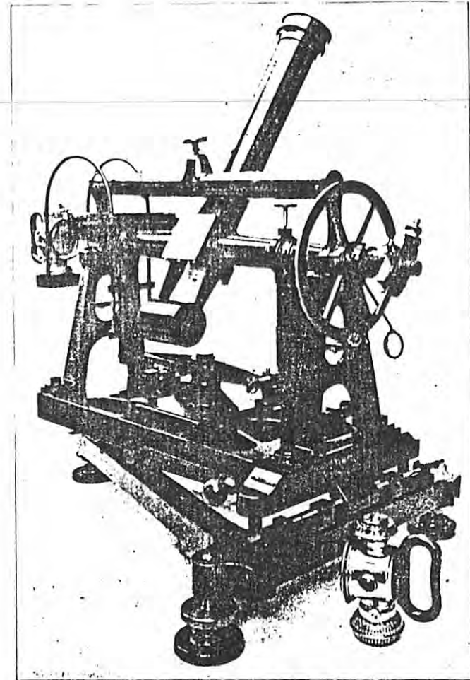
Broken-Back Transit, Navy Pattern.
