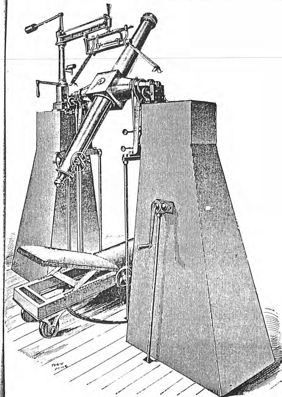
Prime Vertical Transit.
