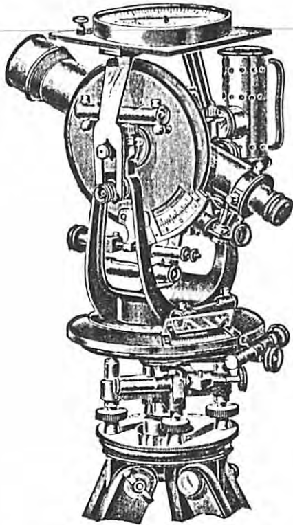
Four-inch Mining Transit.
