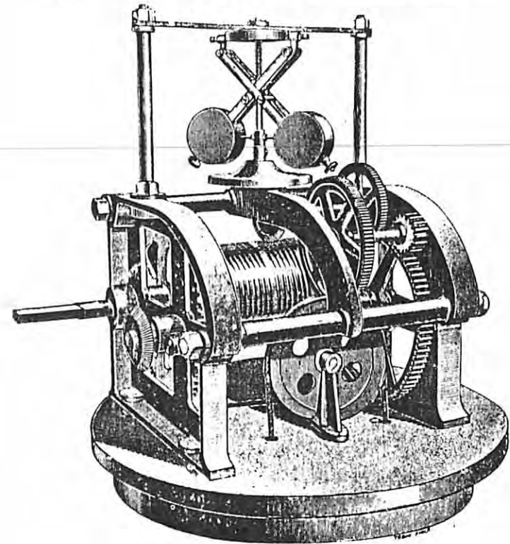
Equatorial Driving-Clock.
