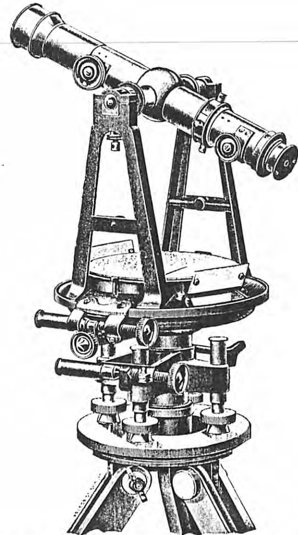
5-inch and 6-inch Plain Mining Transit, No. 1.
