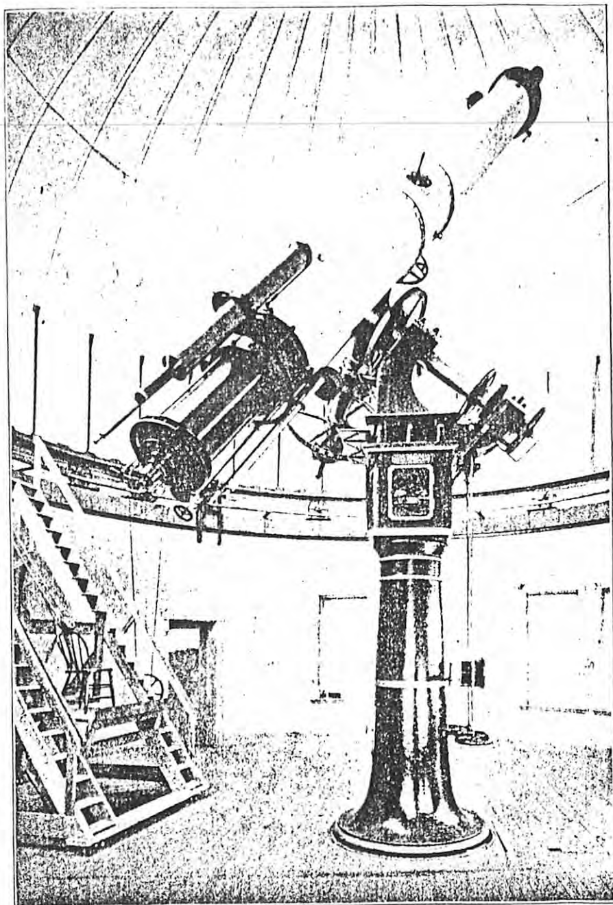
Denver Equatorial, 20 inches Aperture. Designed and constructed by G. N. Saegmuller, Washington, D. C.
