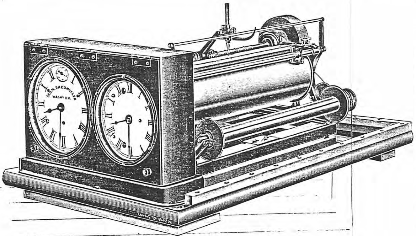
Coast Survey Tide Gauge.
