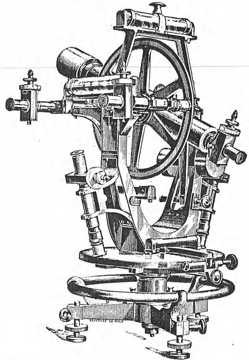
10-inch Altitude-Azimuth.
