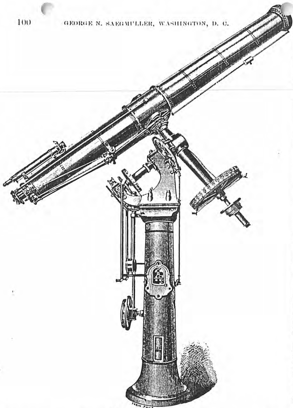
12-inch Equatorial.
