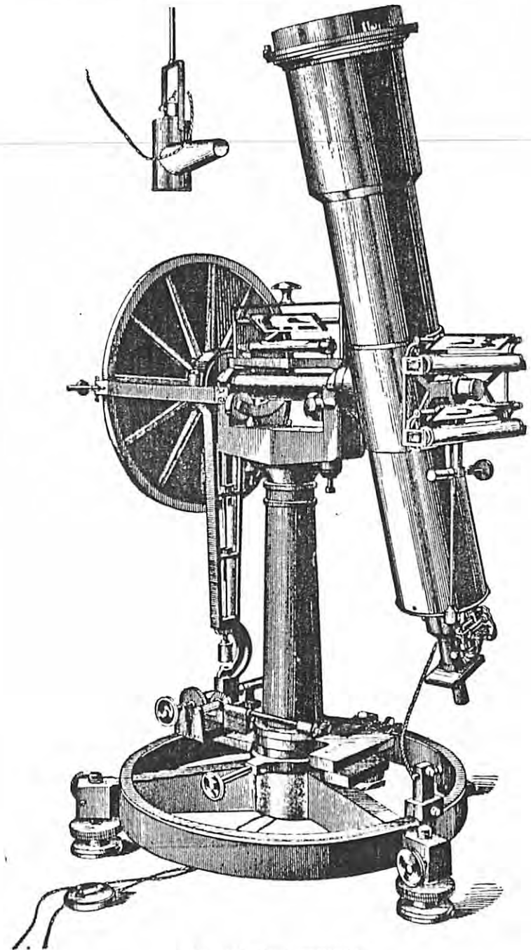
Zenith Instrument.
