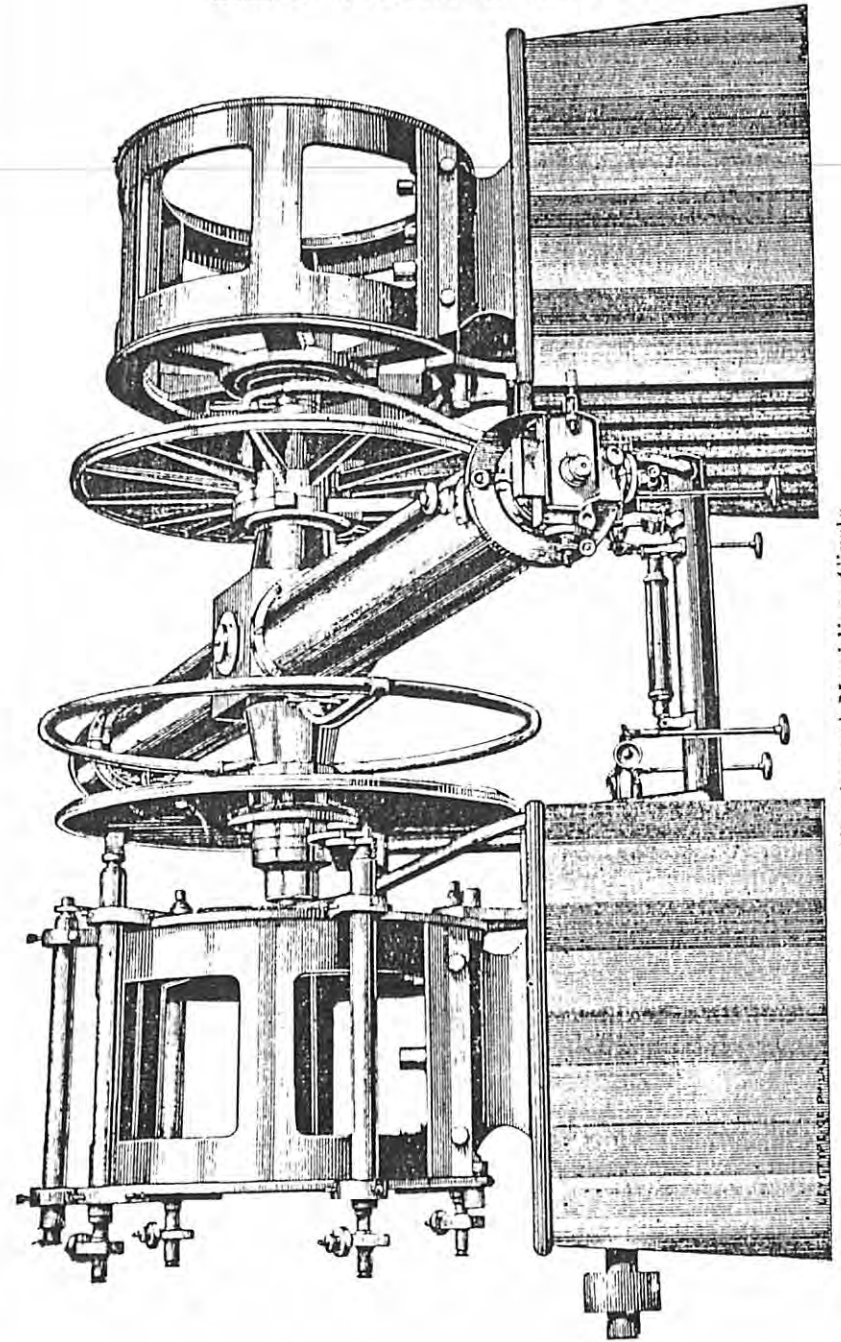
Cincinnati Meridian Circle.
