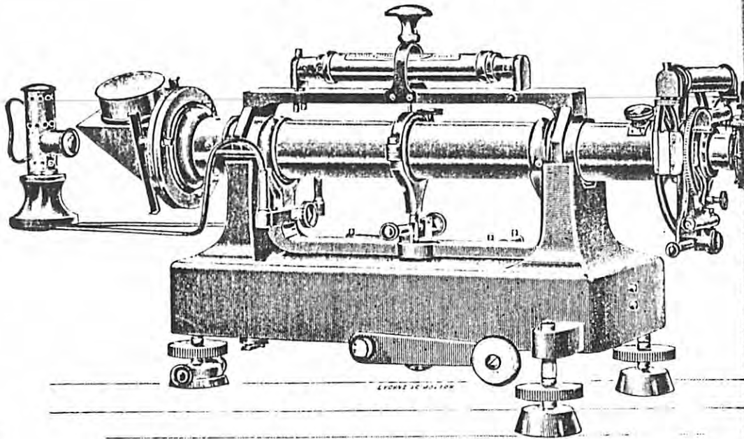
Improved Prismatic Transit.
