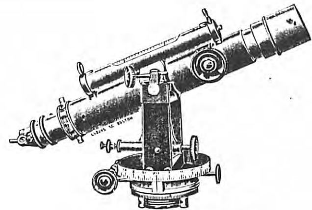
Saegmuller Solar with Hour Circle.
