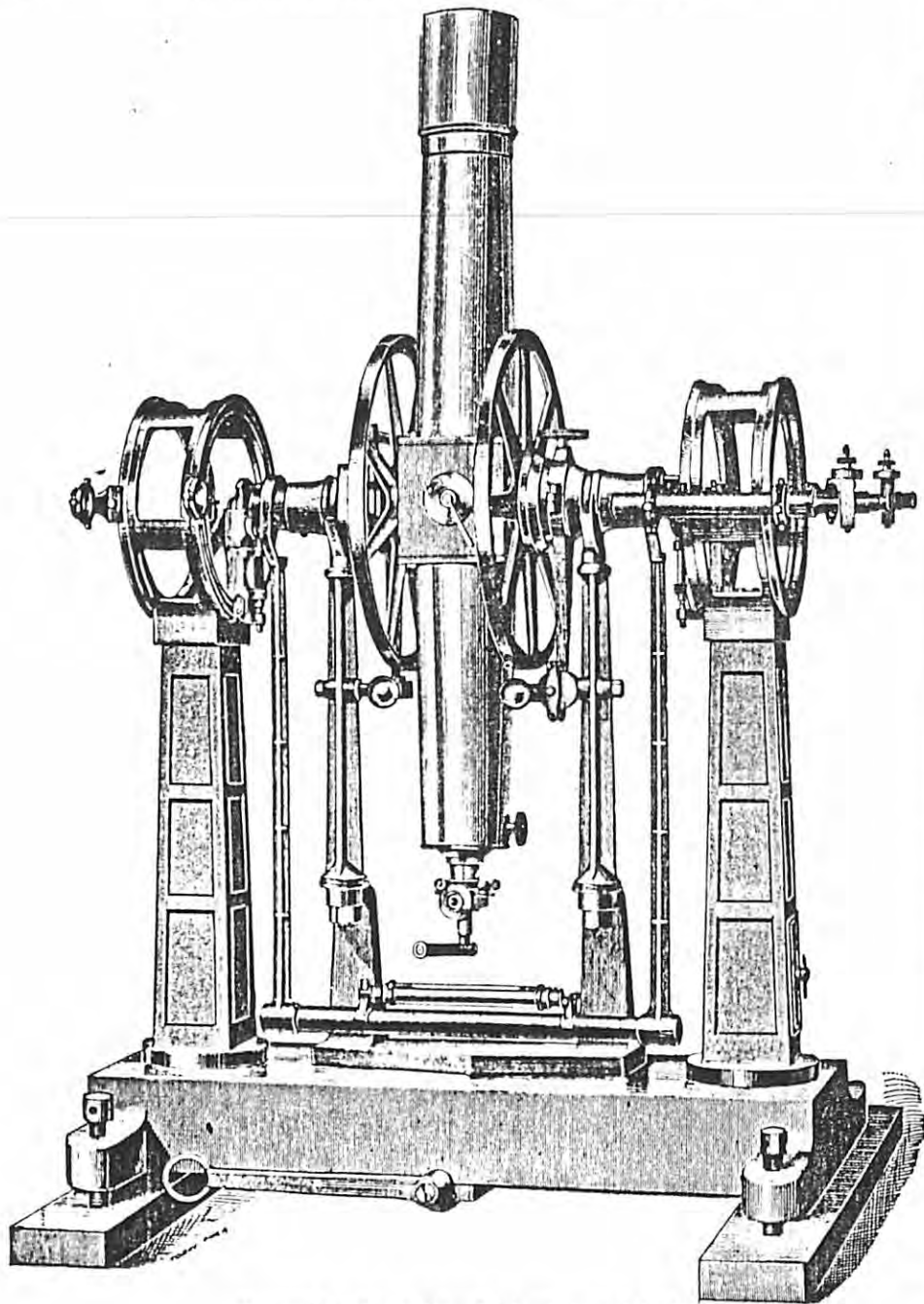
4- and 5-inch Steel Meridian Circle.
