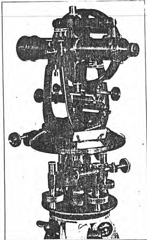
Four-inch Mining Transit.
