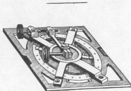
CLEAVER PROTRACTOR
