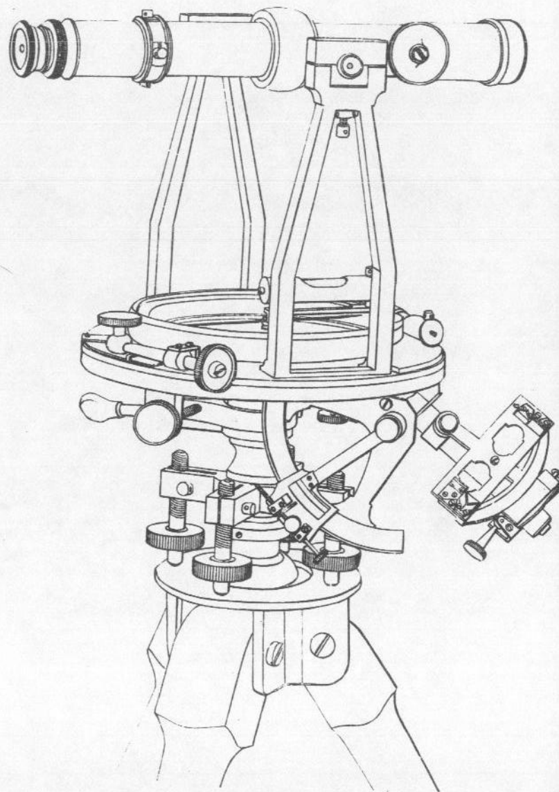
SOLAR TRANSIT. No. 6. Plain.
