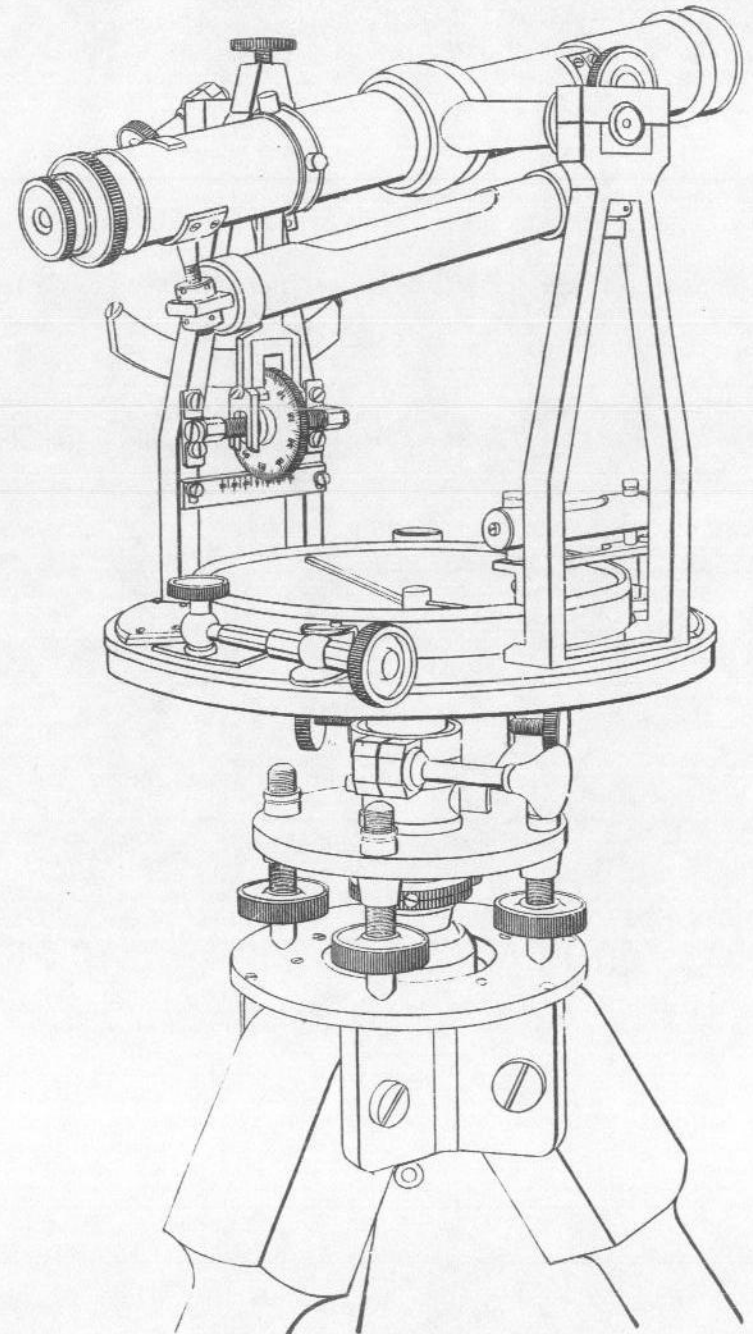
NO. 7.—WITH GRADIENTER, LEVEL TO TELESCOPE, AND VERTICAL ARC.
