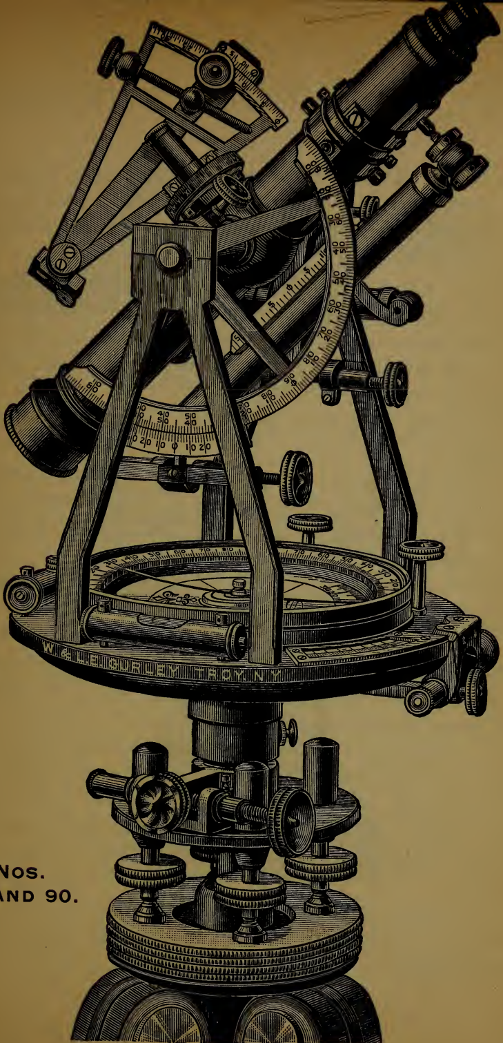
SURVEYORS' TRANSIT WITH SOLAR ATTACHMENT.
