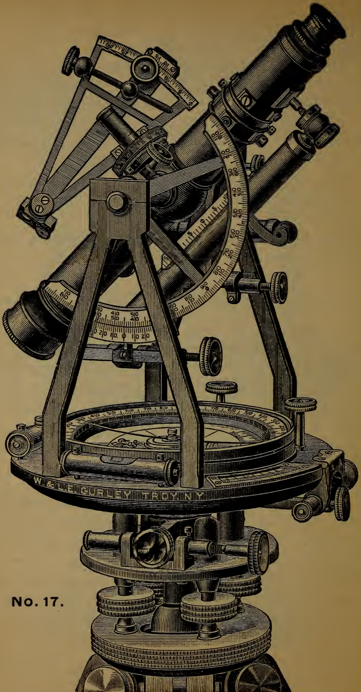
ENGINEERS' TRANSIT, WITH SOLAR ATTACHMENT. Price as shown, $250.00.
