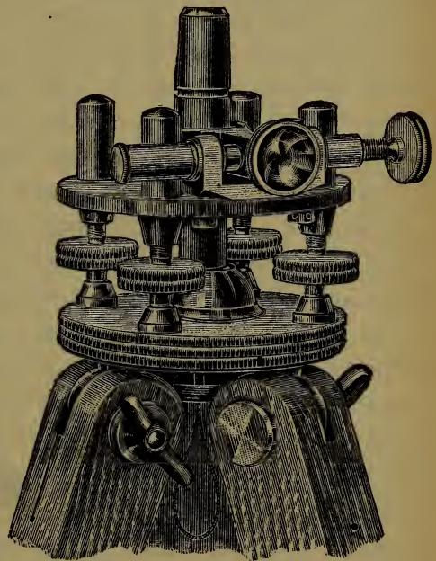
NOS. 176 AND 242. LEVELING-HEAD.
