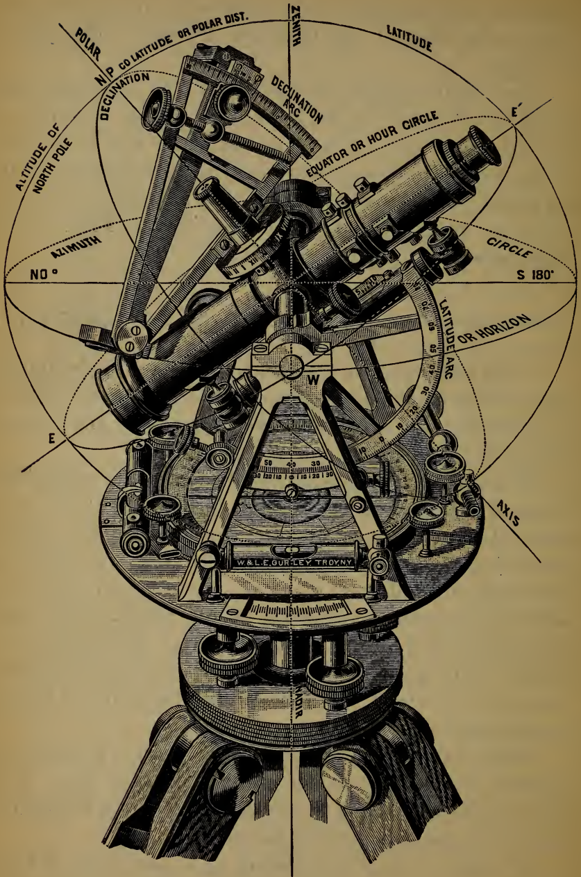
GRAPHIC ILLUSTRATION OF THE SOLAR APPARATUS
