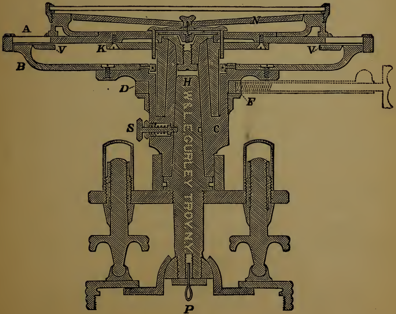
THE SOCKETS AND CIRCULAR PLATES.
