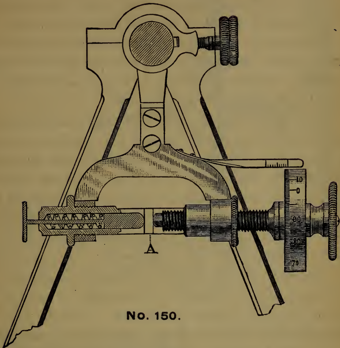
GRADIENTER ATTACHMENT. Price, $18.00.
