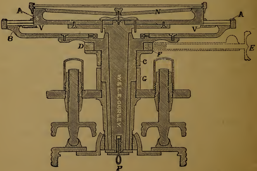
THE SOCKETS AND CIRCULAR PLATES.
