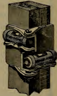
ROD-LEVEL AS APPLIED TO A ROD.
