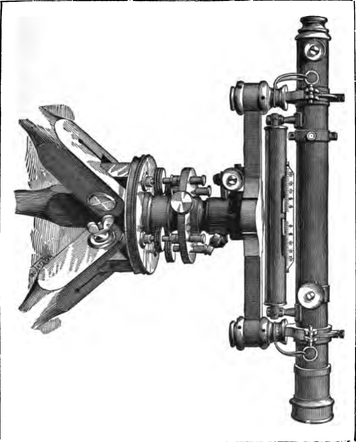
IMPROVED 17" IN. Y LEVELING INSTRUMENT.
