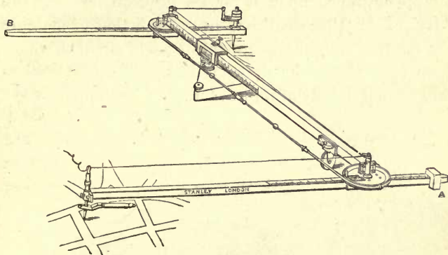
Improved Eidograph.
