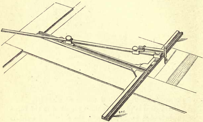
Conchoidograph.
