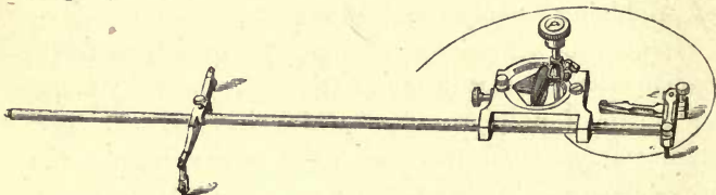
Penrose and Bennett's Helicograph.
