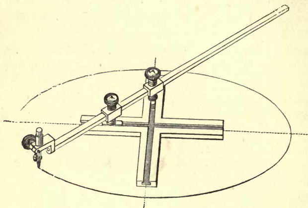
Elliptic Trammel.
