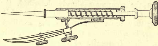
Pump Bow.
