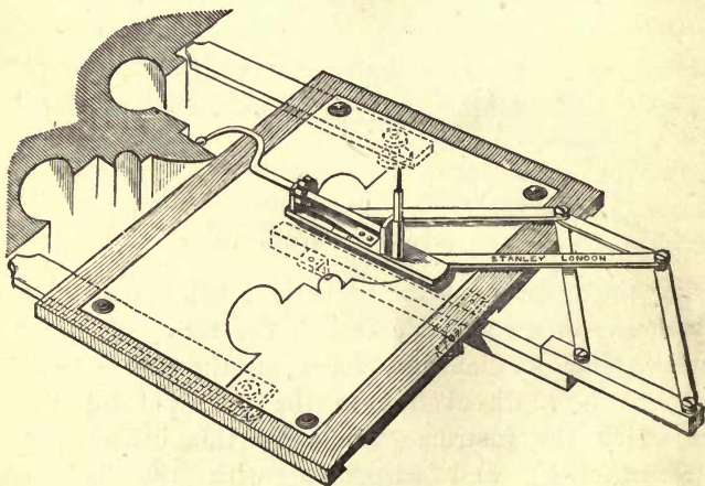
Willis' Cymograph.
