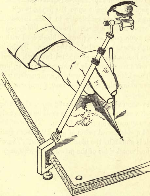
Wollaston's Prismatic Camera Lucida in use.
