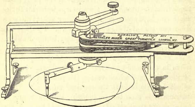
Burstow's Patent Elliptograph.
