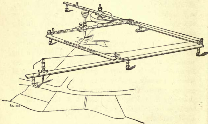
Pantagraph.
