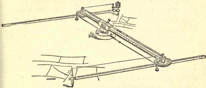
Eidograph.
