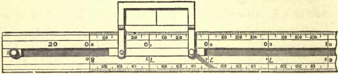
Computing Scale.
