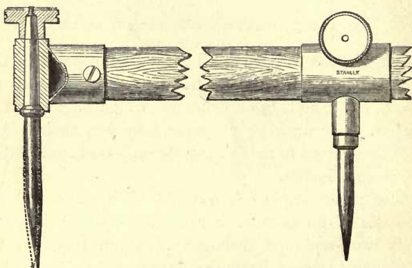
Colonel Strange's Adjusting Beam Compasses.
