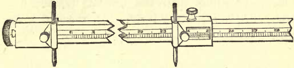
Divided Beam Compasses (Ordnance Pattern).
