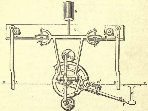
Amsler's Integrater.
