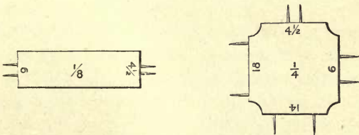
Brick Gauges.
