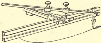
Semi-elliptic Trammel.
