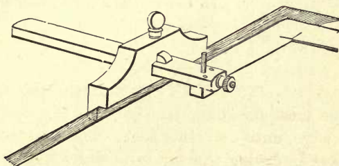
Cutting Gauge to remove Paper from Drawing-board.
